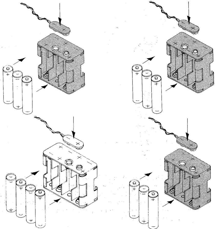
BATTERY-PACK ILLUSTRATION
