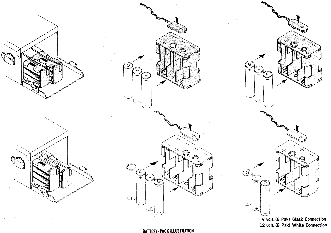
BATTERY-PACK ILLUSTRATION
