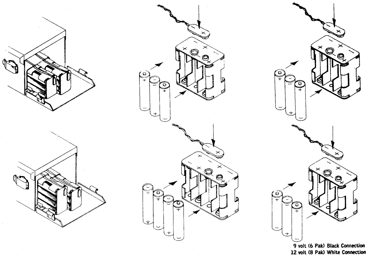
BATTERY-PACK ILLUSTRATION
