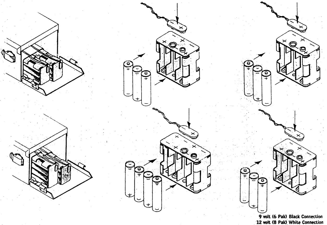
BATTERY-PACK ILLUSTRATION
